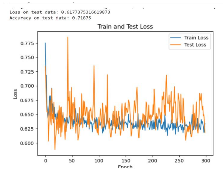
Figure 11. Best Neural Networks Model
